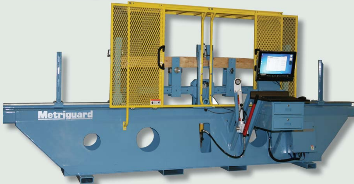
Metriguard Model 312 Bending Proof Tester
